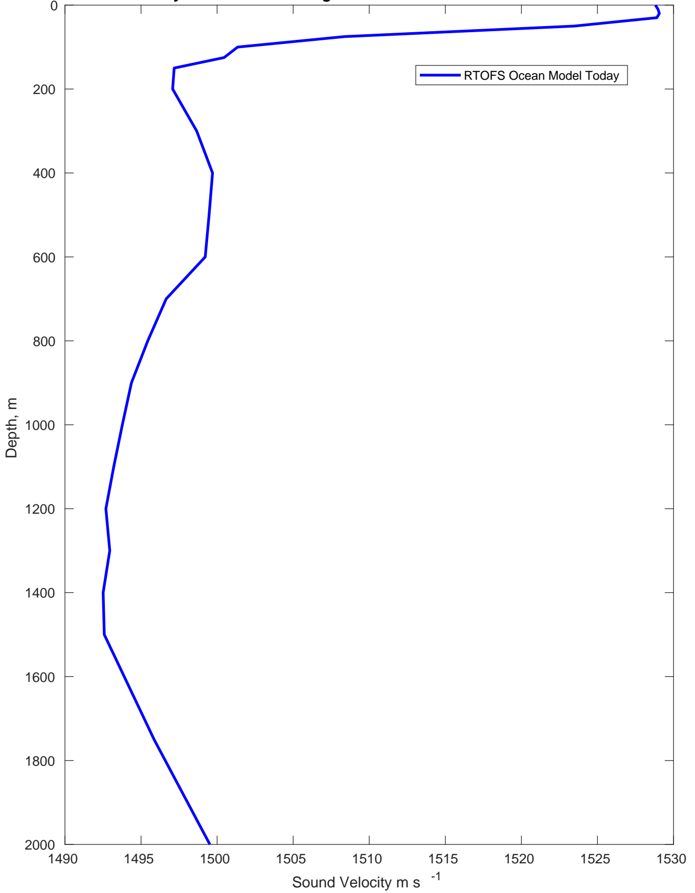
Sound Velocity Profile for BP Senegal YT Offshore on 02-Feb-2022 00:00:00
